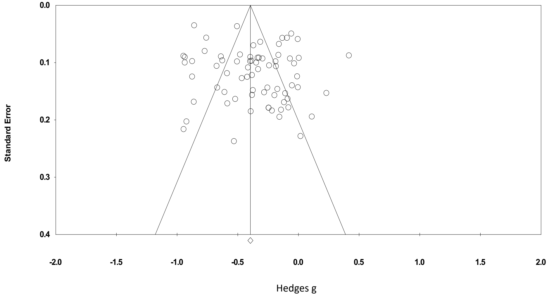
Funnel Plot of Standard Error by Hedges g
