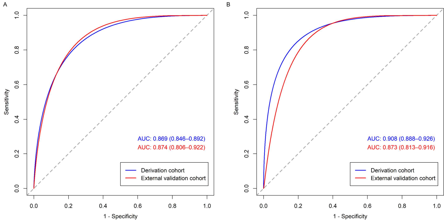
Figure S5. Receiver operating characteristic curves of the extreme gradient boosting models for cardiac surgery–associated acute kidney injury stages 2-3. (A) Receiver operating characteristic curve of the extreme gradient boosting model with only the preoperative variables. (B) Receiver operating characteristic curve of the extreme gradient boosting model with the preoperative and intraoperative variables. AUC, area under the curve.
